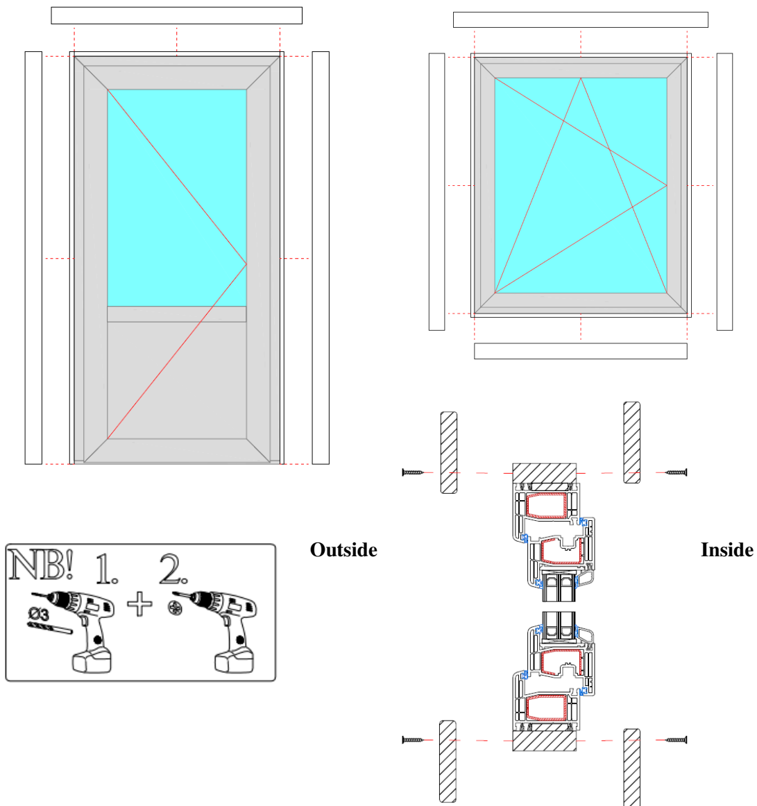
Figure 1 – Facial board installation:
